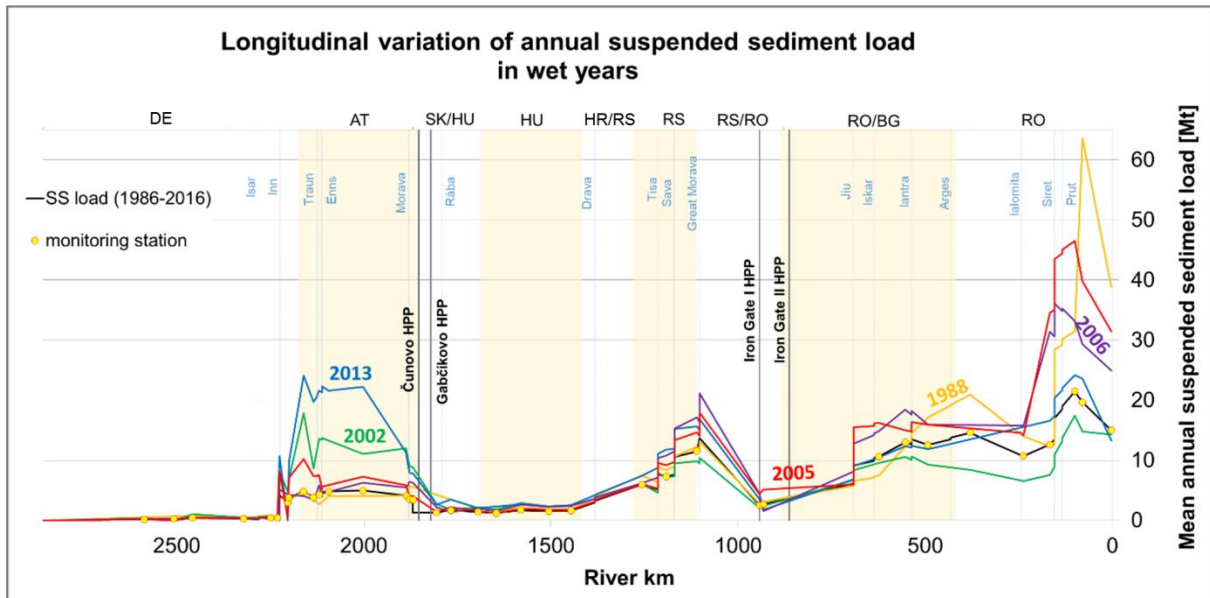
Longitudinal variation of annual suspended sediment load along the Danube River in wet years (BME, 2019)
